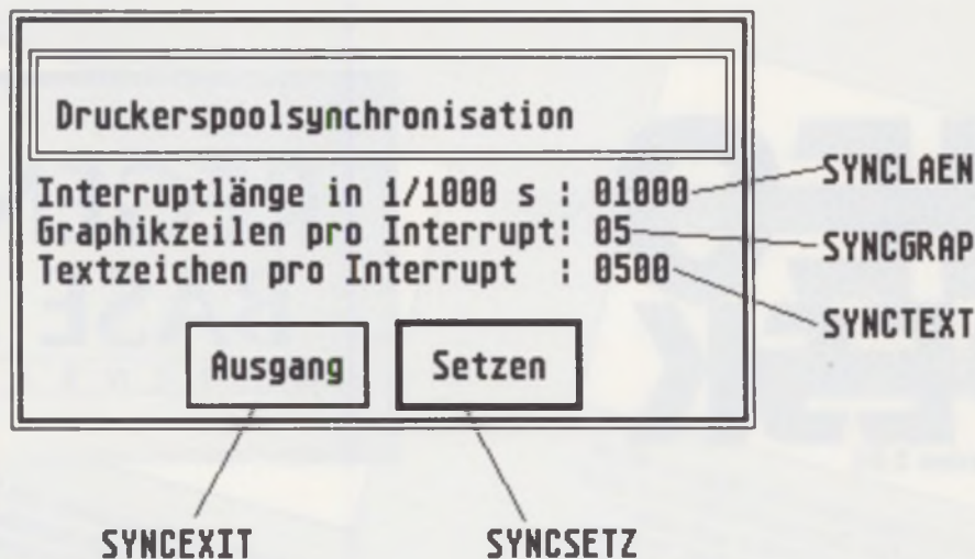
Abb. 6: Dialog "SYNCHRO"
